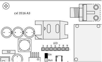
Position LED 3–9
